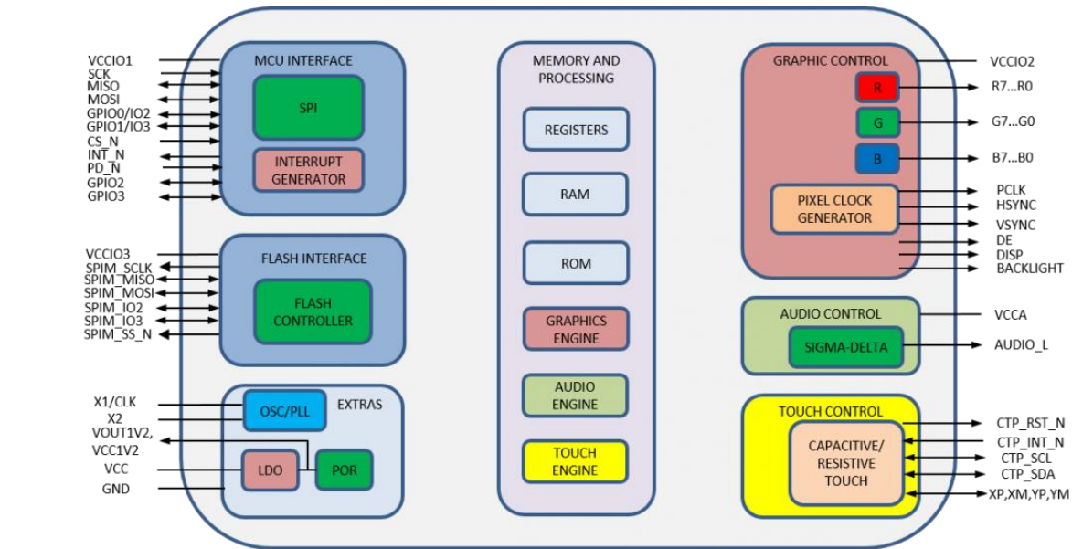
Figure 8. BT817Q Block diagram
